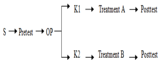
Figure 1 Research Design
